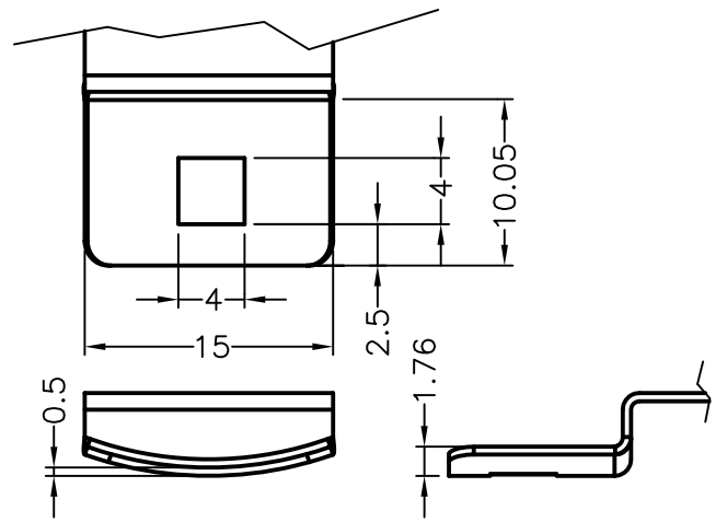
ASSEMBLY PART
